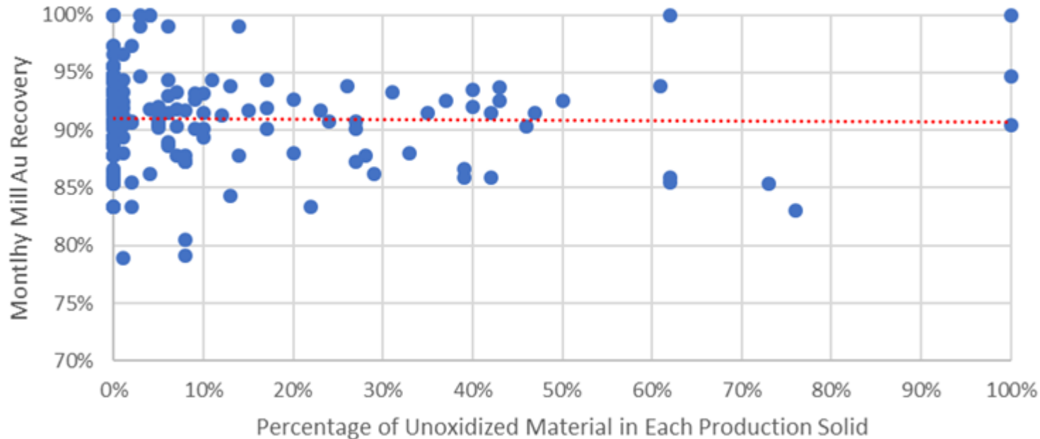
Monthly Mill Au Recovery vs Percentage of Unoxidized Material in DeLamar Production Areas
