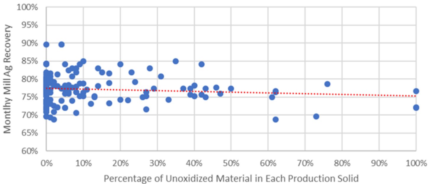
Monthly Mill Ag Recovery vs Percentage of Unoxidized Material in DeLamar Production Areas
